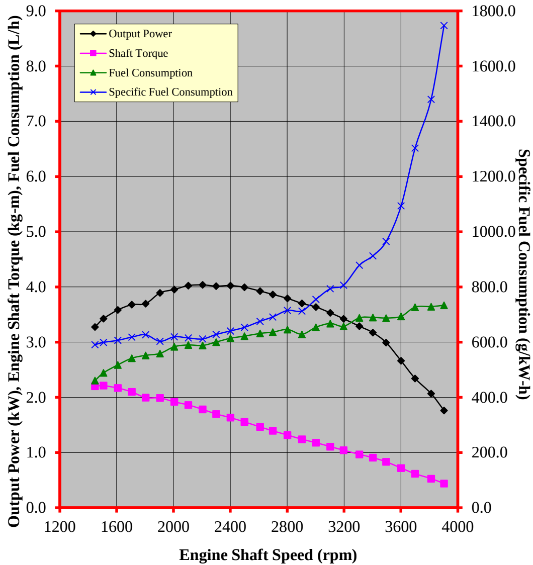
Figure 3. Performance characteristic curves of the BRIGGS & STRATTON B18 327431 Gasoline Engine
