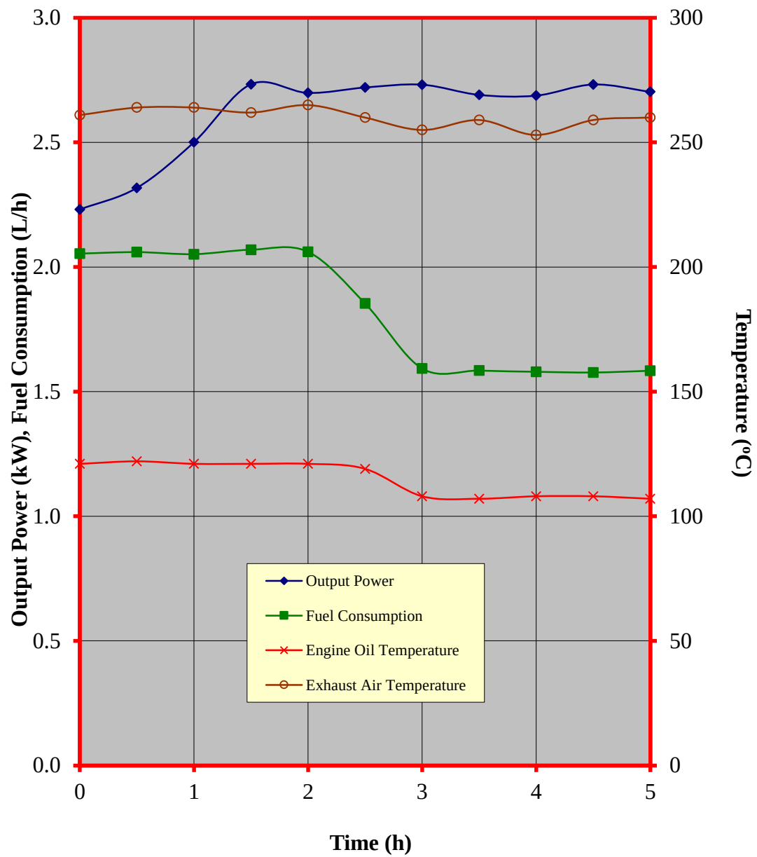
Figure 4. Performance characteristic curves during the continuous running test of the BRIGGS & STRATTON B18 327431 Gasoline Engine
